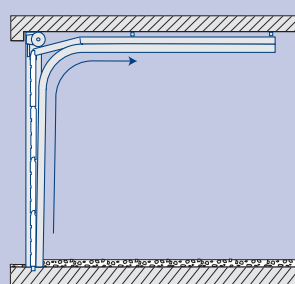
Sectional Operating Gear
