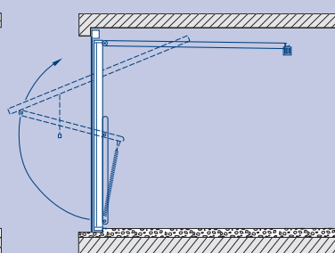
Retractable Operating Gear
