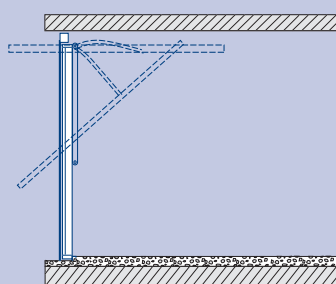
Canopy Operating Gear
