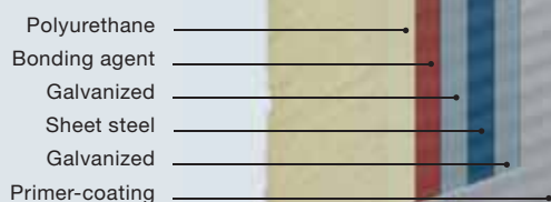
Door leaf construction
