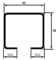
Top Track
