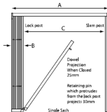
Single Sash
